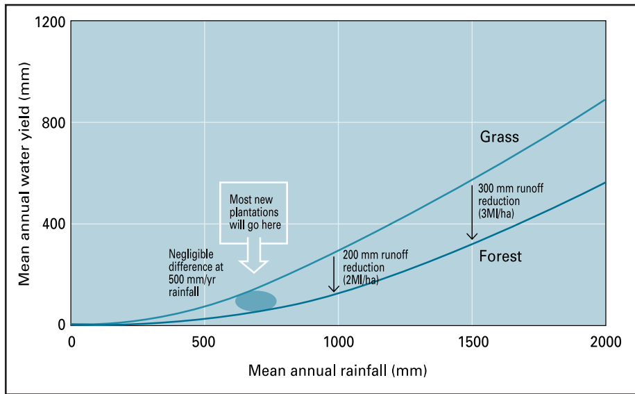
FIGURE 2 Water Yield is Higher from Grassed Catchments than Forests.
