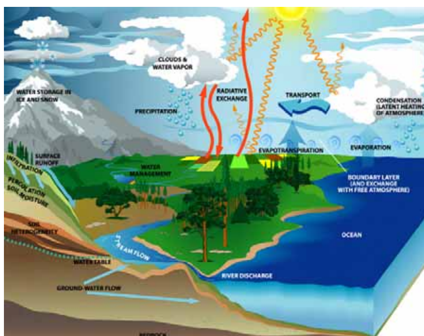
FIGURE 1 The Hydrological Cycle of Water Through the Environment.
